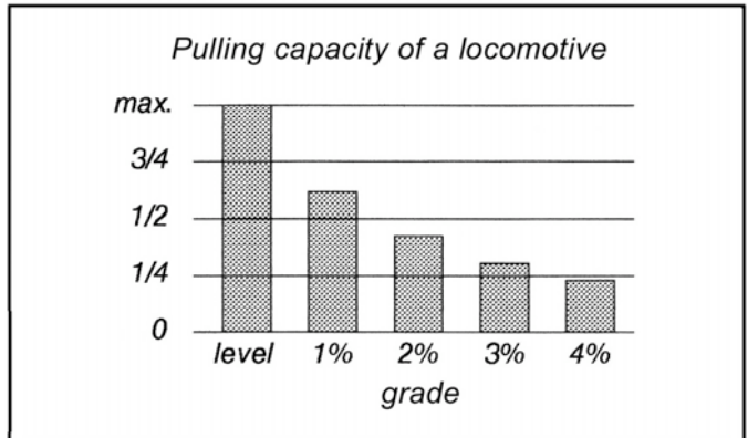
Figure 7 • Operation on Grades
