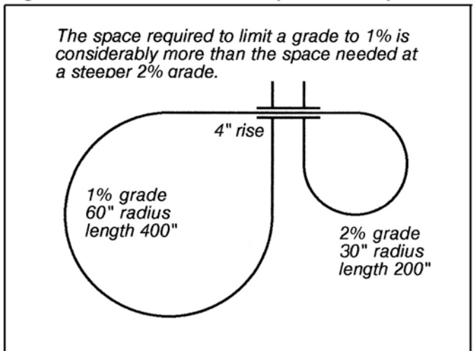
Figure 8 • Gentle Grades Require More Space
