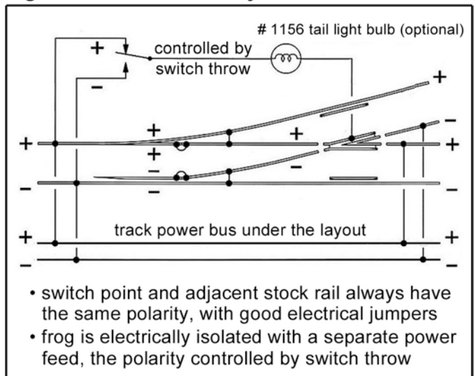
Figure 17 • DCC friendly & ideal DC turnout
